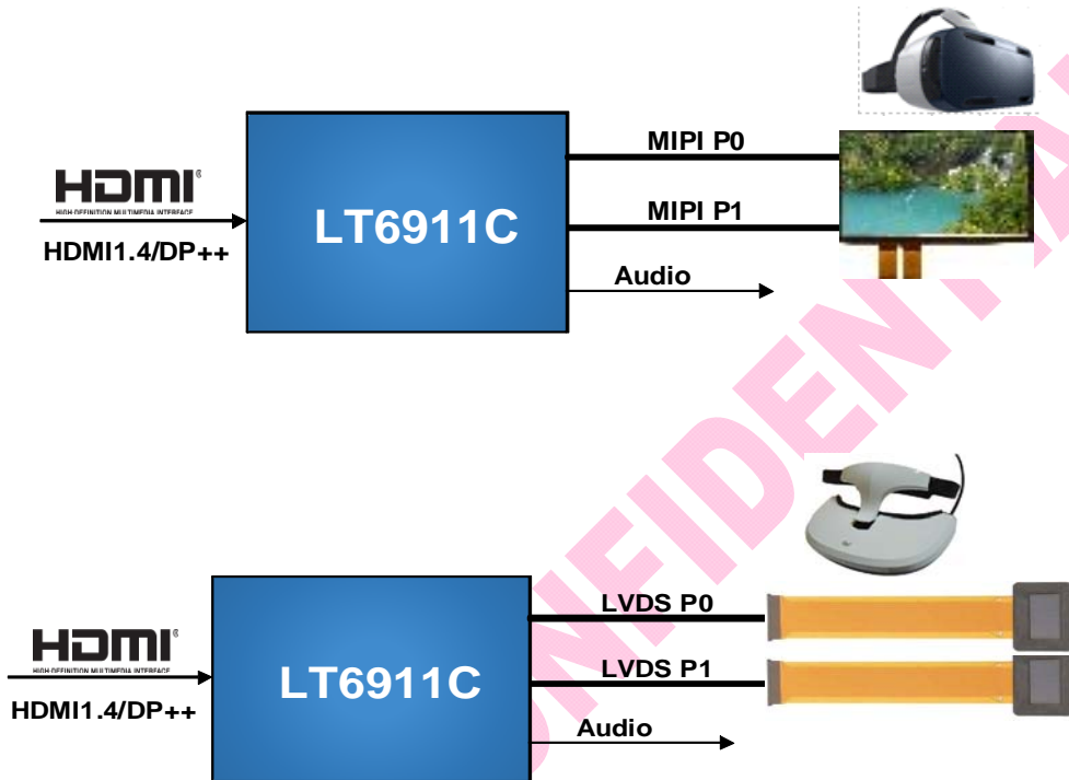
Figure3.1 Application Diagrams
